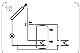
Standard solar system with heat dump (page 43)
