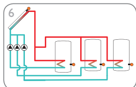
3-store solar system with pump logic and heat exchange control (page 23)
