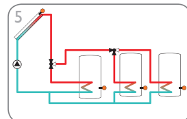
3-store solar system with valve logic and heat exchange control (page 20)
