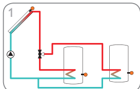
2-store system with valve logic, 1 pump, 3 sensors and 3-port valve (page 8)
