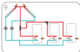
3-store solar system with east-/west collectors (page 32)
