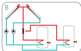
Solar system with east-/west collectors and 2 stores (valve logic) (page 29)
