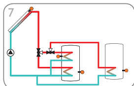
Solar system with store loading in layers and 2 stores (page 26)
