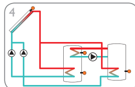
2-store solar system with pump logic and heat exchange control (page 17)
