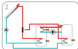
2-store solar system with valve logic and heat exchange control (page 11)
