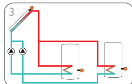
2-store solar system with pump logic (page 14)
